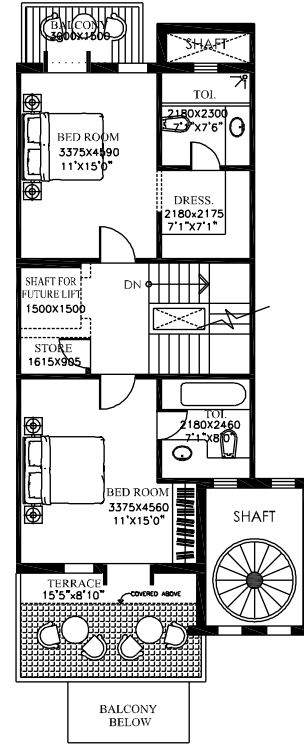
TENTATIVE SECOND FLOOR PLAN
