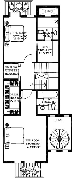
TENTATIVE FIRST FLOOR PLAN
